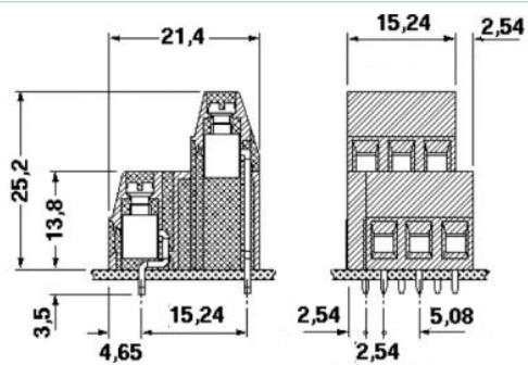
Dimensioned drawing
