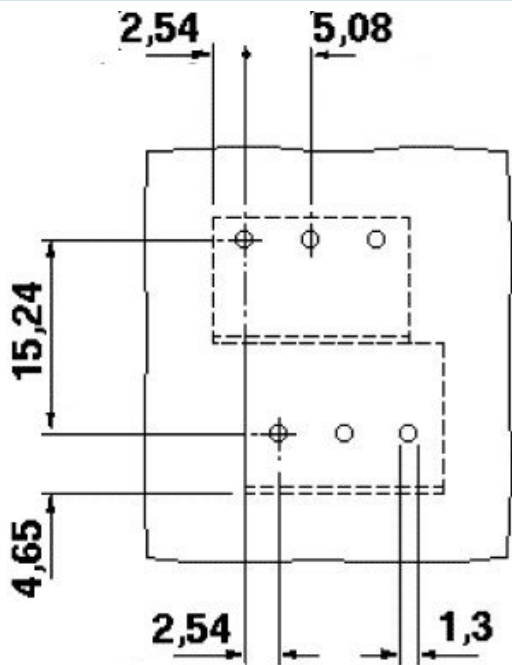
Drilling diagram
